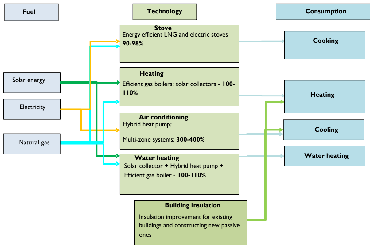
Fig. 15. Technology and corresponding efficiency recommendations for technologies that should be implemented in the Fifth Technological Zone
