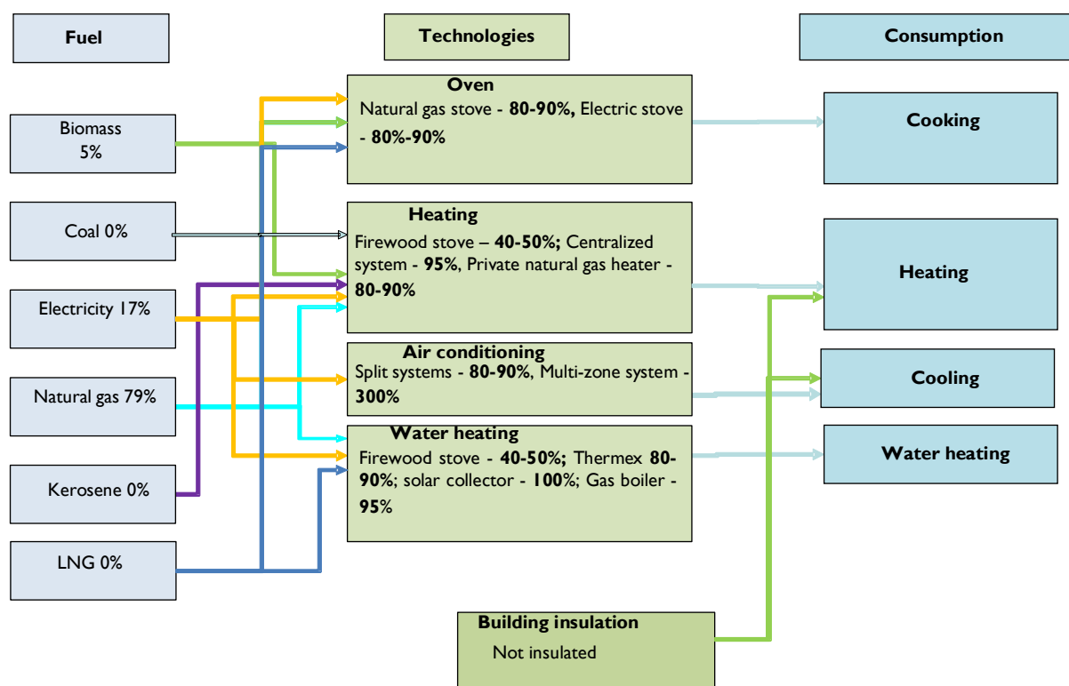
Fig. 14. Available technologies and their efficiency in the Fifth Technological Zone
