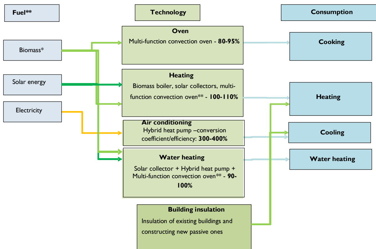
Fig. 7. Technology and corresponding efficiency recommendations for technologies that should be implemented in the First Technological Zone
