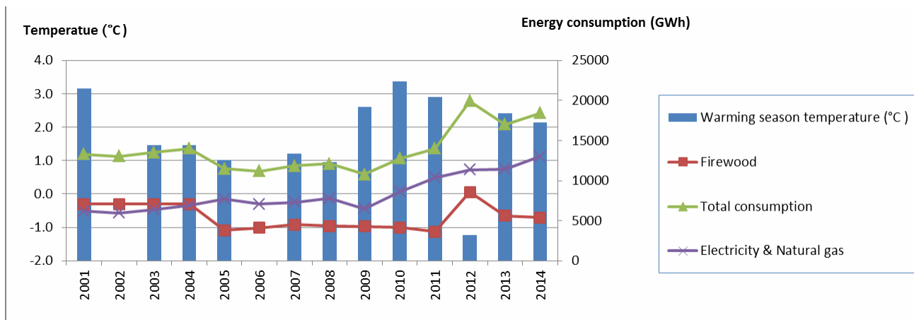
Fig. 21. Correlation between energy consumption and warming temperature
