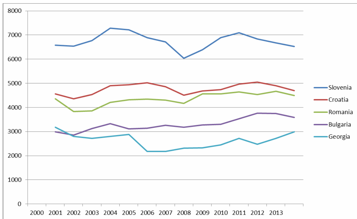
Fig. 16. Energy consumption per capita in residential buildings of Georgia and EU countries
