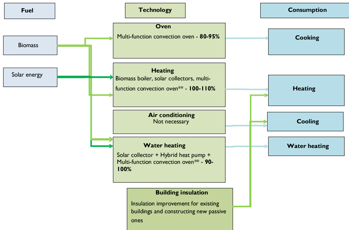
Fig. 11. Technology and corresponding efficiency recommendations for technologies that should be implemented in the Third Technological Zone
