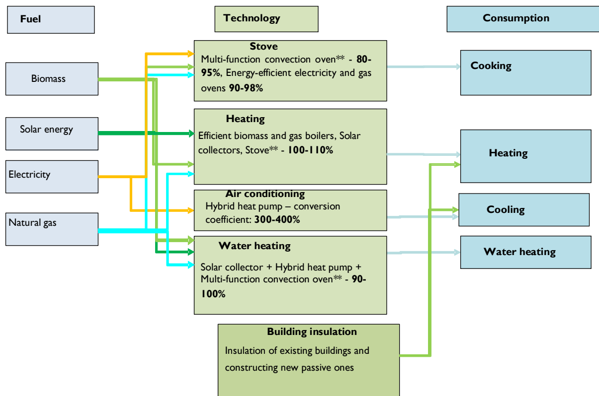
Fig. 13. Technology and corresponding efficiency recommendations for technologies that should be implemented in the Fourth Technological Zone
