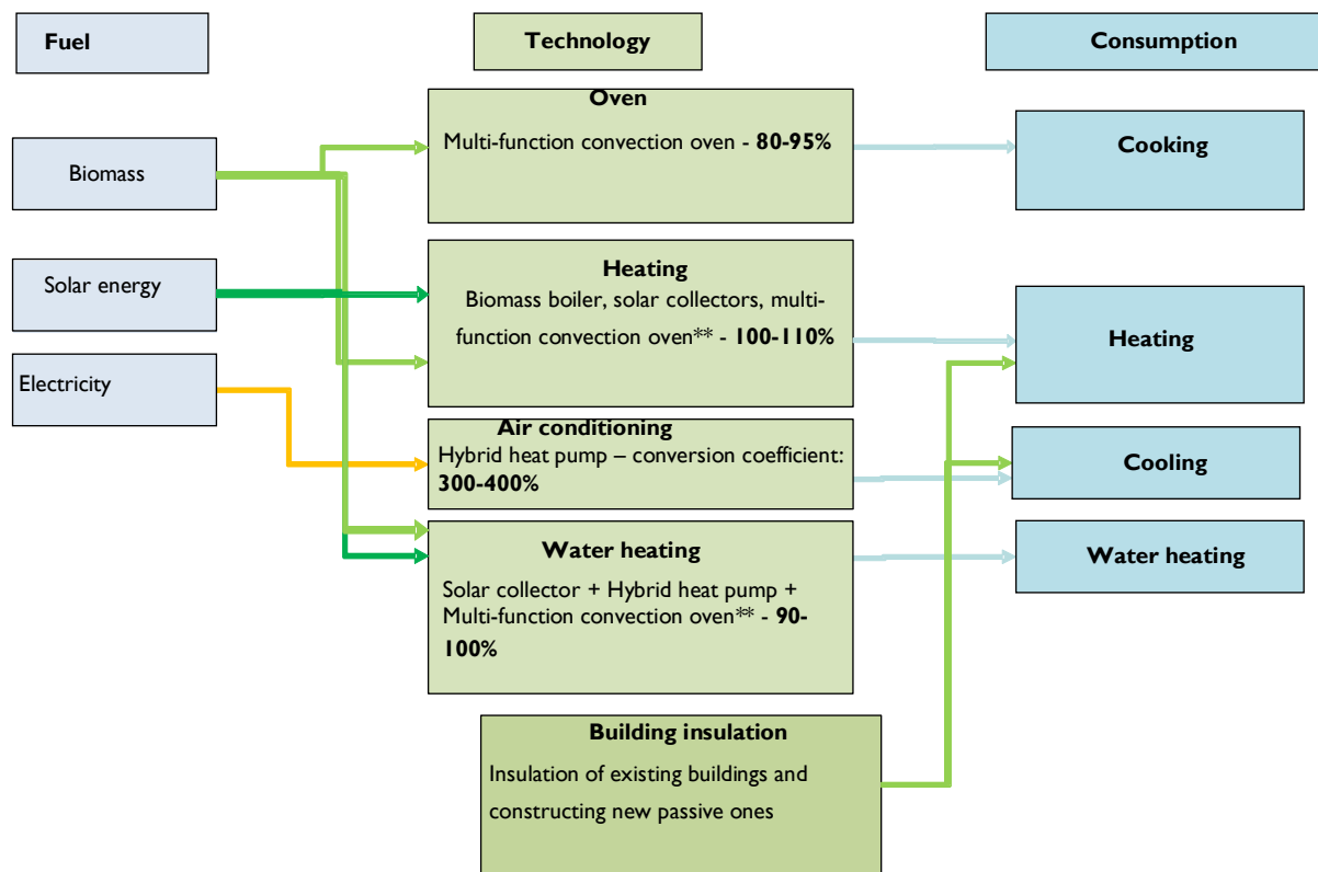
Fig. 9. Technology and corresponding efficiency recommendations for technologies that should be implemented in the Second Technological Zone
