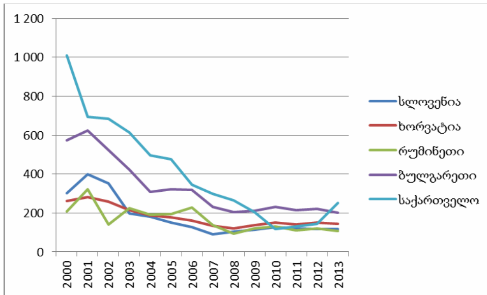
Fig. 17. Energy consumption per 1 USD in non-residential buildings of Georgia and EU countries
