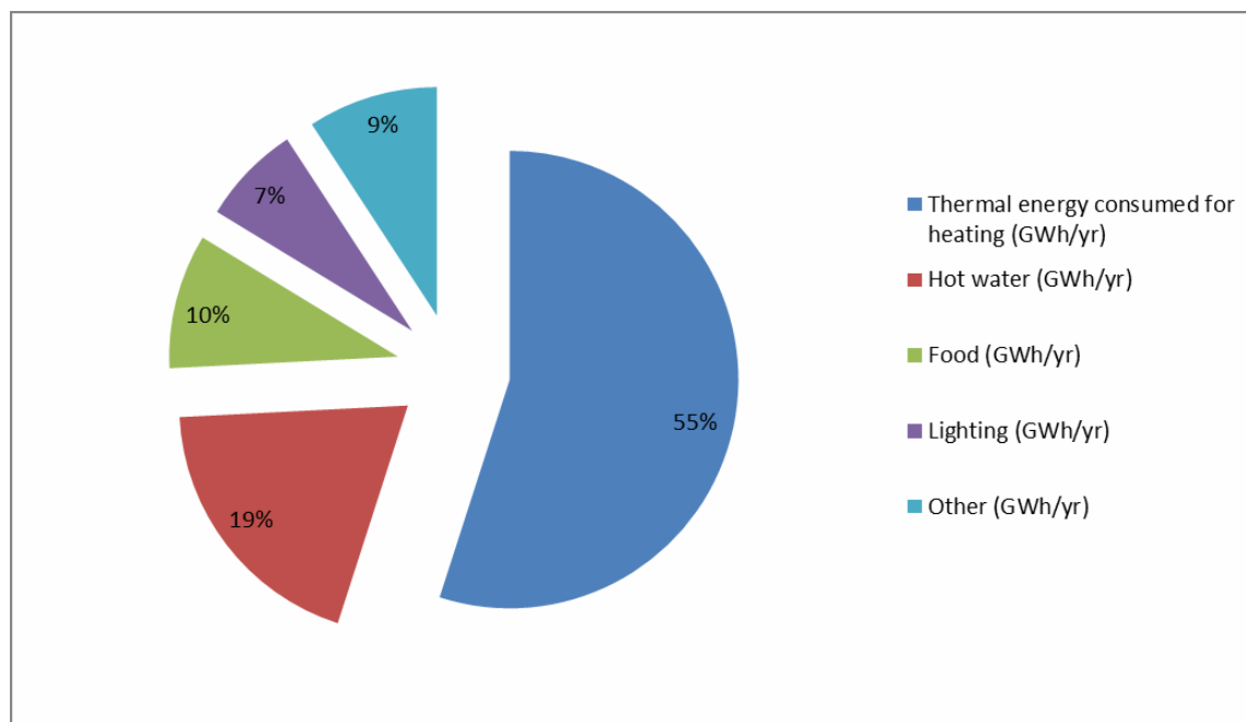
Fig. 27. Distribution of energy consumption by purposes (%)
