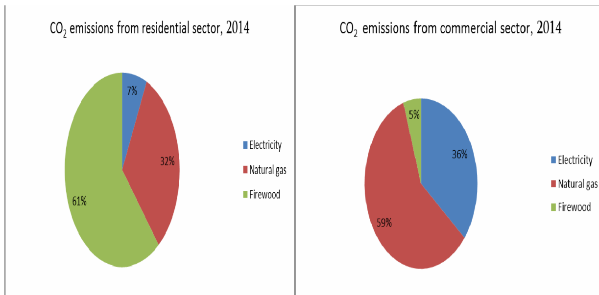
Fig. 23. Distribution of CO 2 emissions in percentages by fuel and building types
